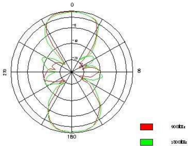
Vertical Pattern
