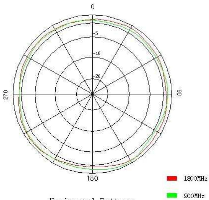
Horizontal Pattern
