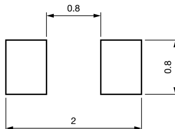
Recommended solder pad footprint
