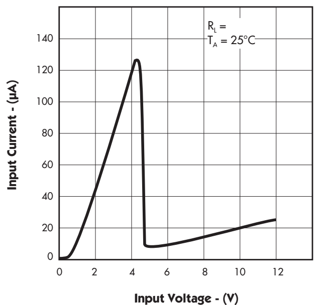
FIGURE 4. — INPUT CURRENT vs. INPUT VOLTAGE
