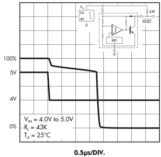
FIGURE 6. — \overline{\text{RESET}} DELAY TIME (HIGH TO LOW)
