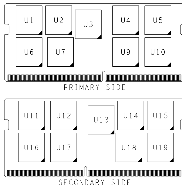
Figure 1: 260-Pin SODIMM
