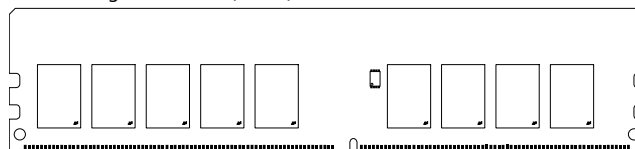
Figure 1: 288-Pin UDIMM (MO-309, R/C-E1)
