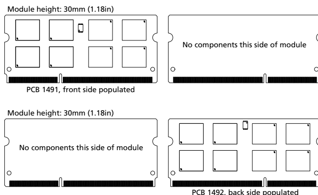
Figure 1: 204-Pin SODIMMs (MO-268 R/C G0, R/C H0)
