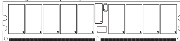
Figure 1: 240-Pin RDIMM (MO-237 R/C K)
