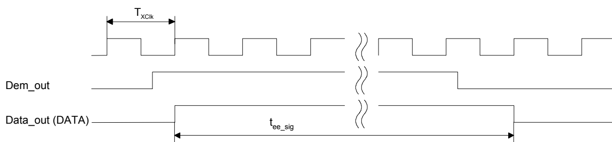
Figure 12. Synchronization of the Demodulator Output
