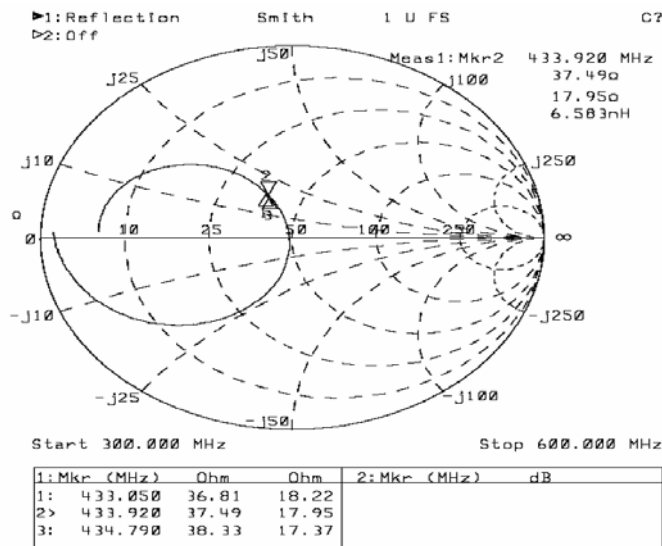
Figure 9. Input Impedance
