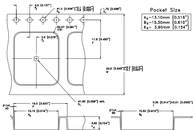
Figure 16. Tape Dimensions
