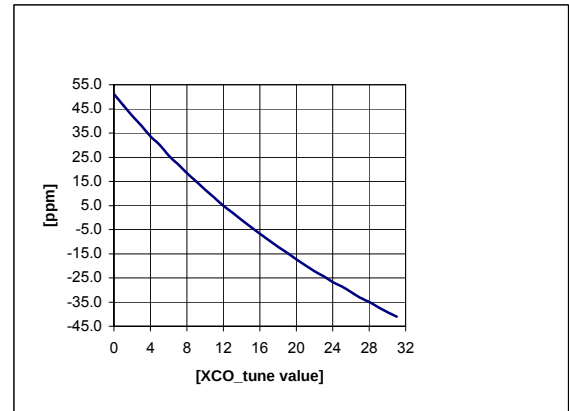
Figure 5. XCO Tuning
