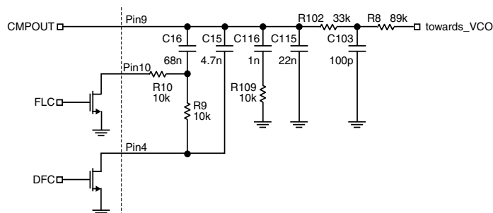
Figure 7. Dual-Loop Filters
