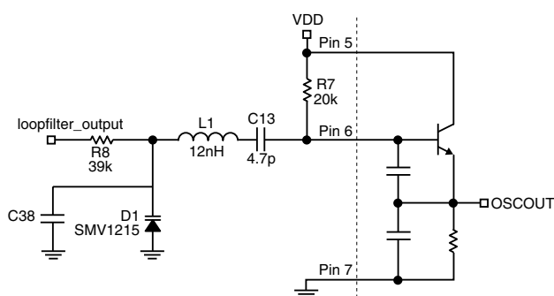
Figure 3. VCO
