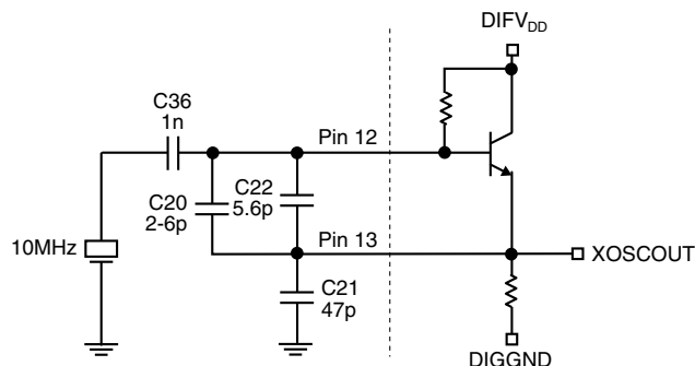
Figure 4. Crystal Oscillator
