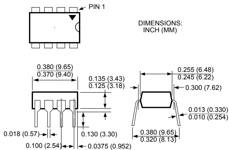
8-Pin Plastic DIP (N)
