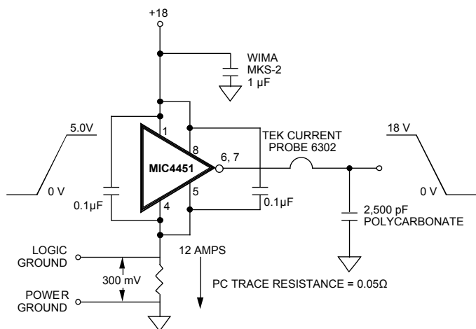
Figure 5. Switching Time Degradation Due to Negative Feedback
