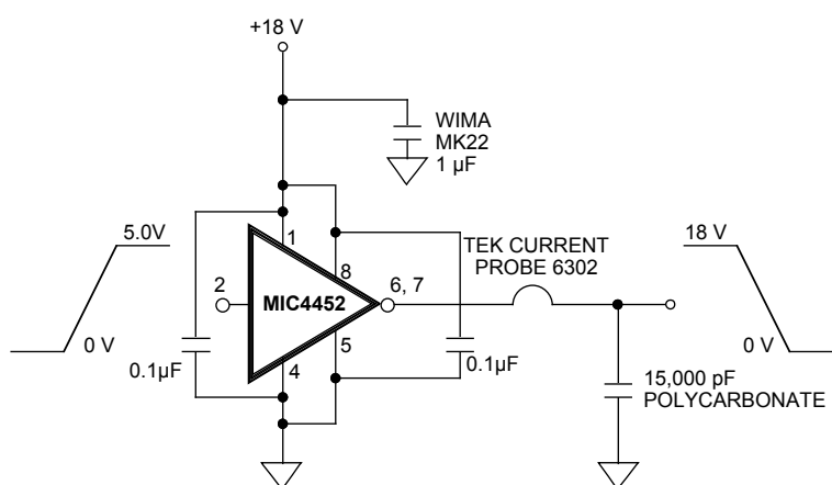
Figure 6. Peak Output Current Test Circuit
