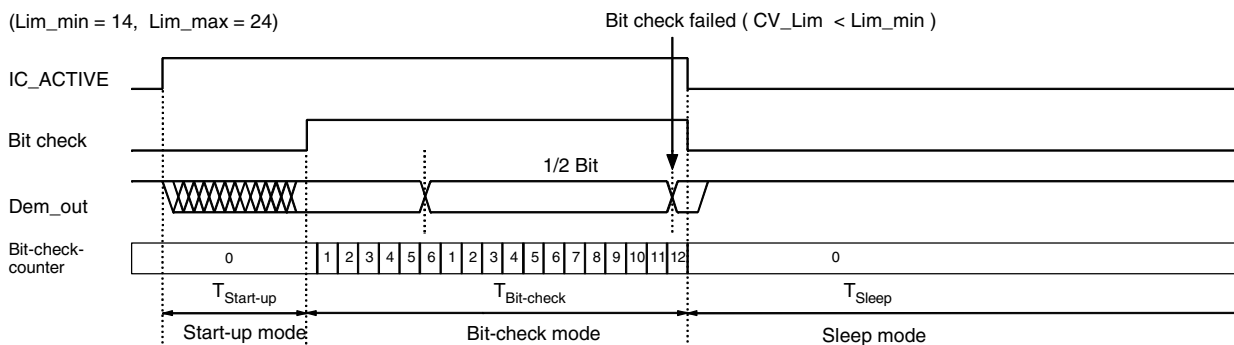
Figure 6-6. Timing Diagram for Failed Bit Check (Condition: \text{CV\_Lim} < \text{Lim\_min} )
