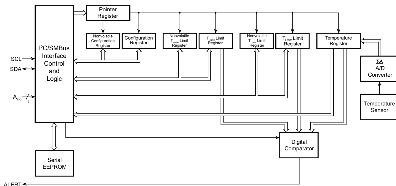
Figure 3-1. Block Diagram
