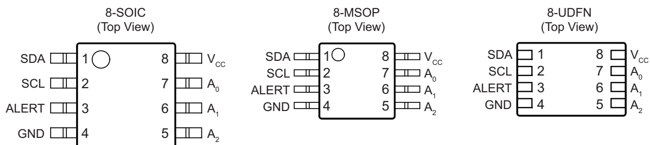
Figure 1. Pin Configurations
