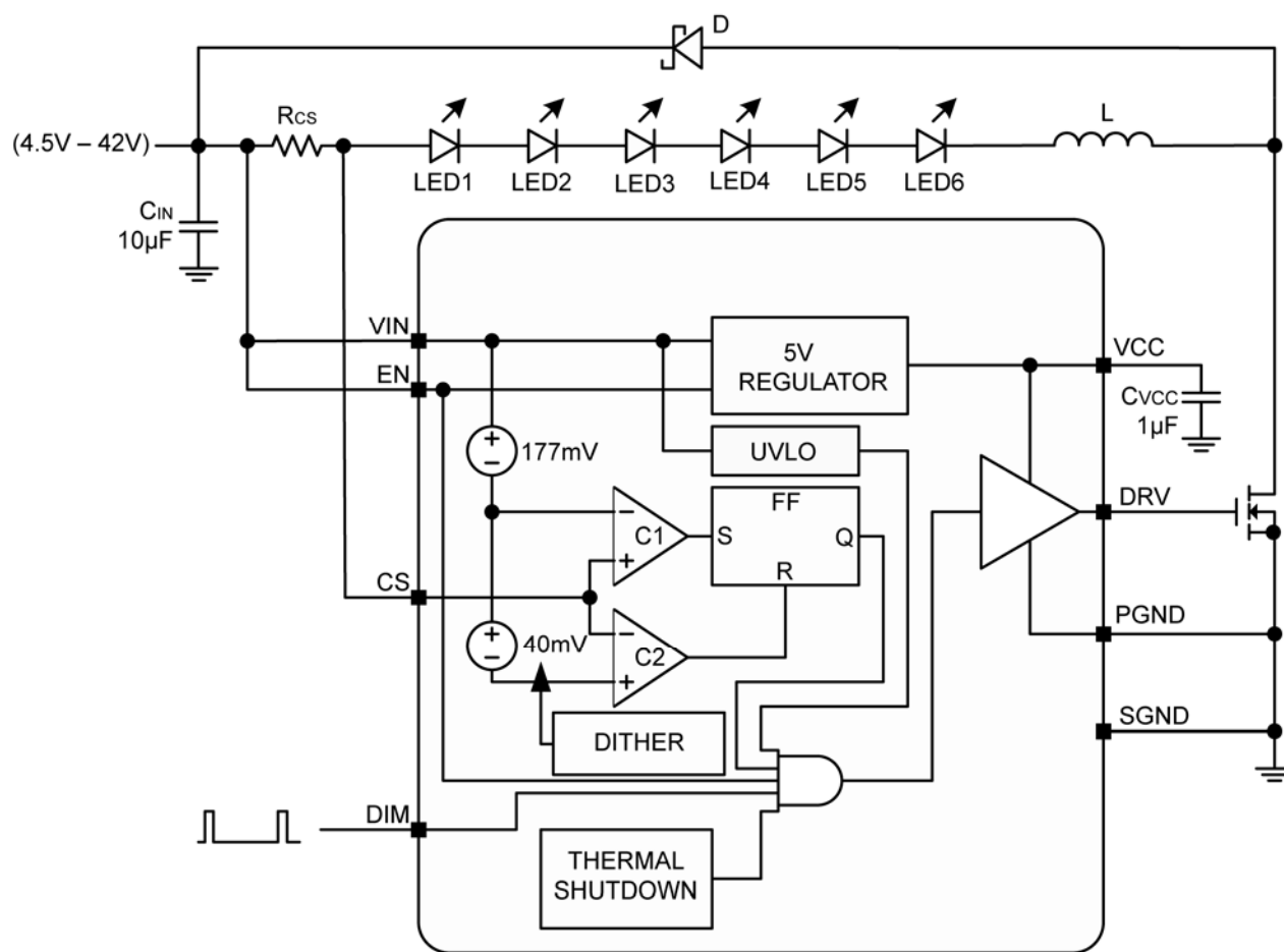
Figure 1. MAQ3203 Block Diagram
