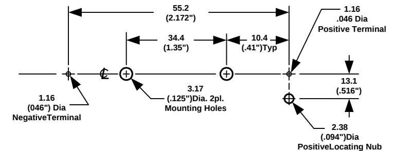
Standard Pc Version P.C. Board Hole layout
