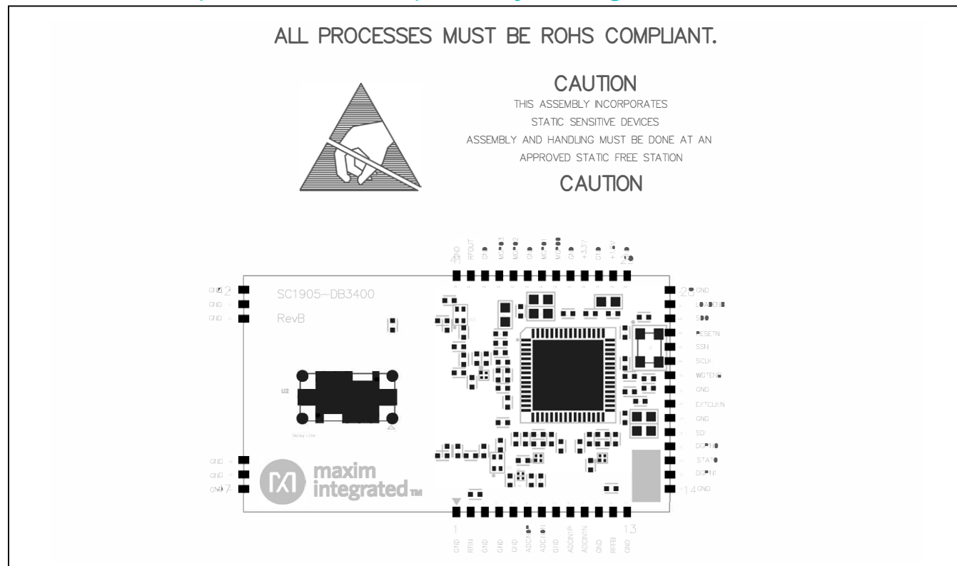
SC1905-DB3400—Assembly Drawing
