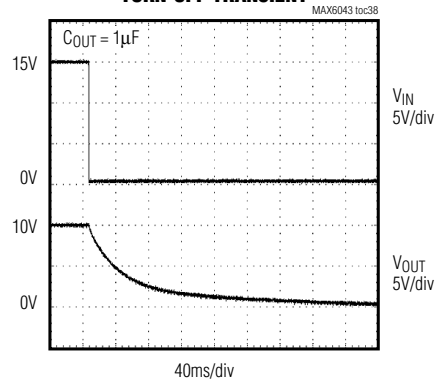
TURN-OFF TRANSIENT
