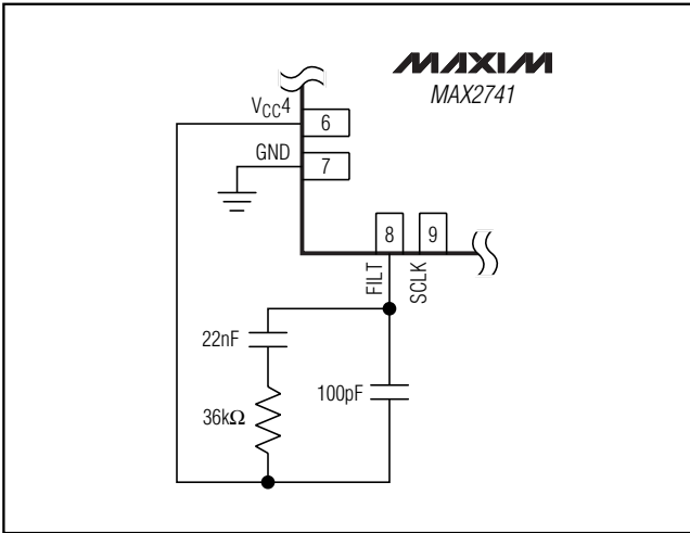
Figure 1. Recommended 3rd-Order PLL Filter
