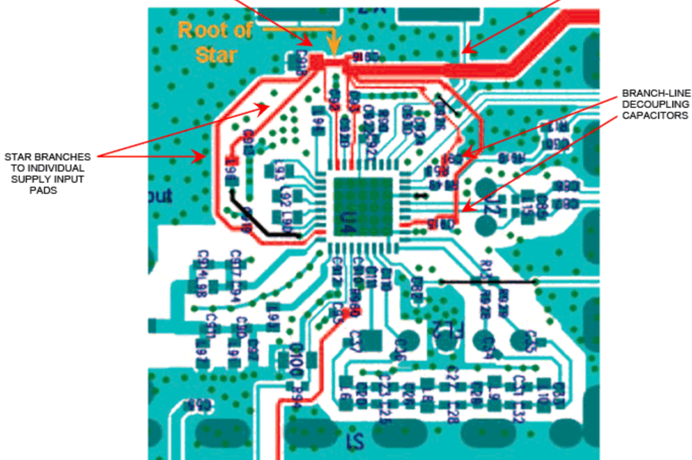
Figure 9. If a component has several supply connections, the power-supply routes can be arranged in a star configuration.
