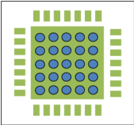
Figure 13. A 5 \times 5 array of via holes embedded in the central ground plane directly under the RF IC.
