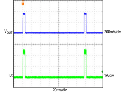
5V OUTPUT, FIGURE 4 CIRCUIT
