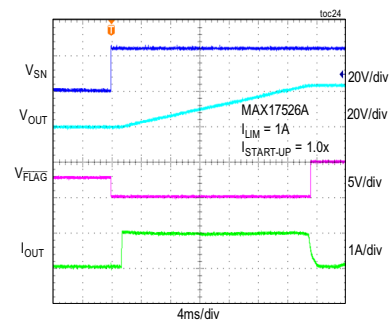
POWER-UP RESPONSE WITH 1000 \mu F CAPACITOR AT NO LOAD
