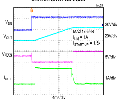
POWER-UP RESPONSE WITH 1000 \mu F CAPACITOR AT NO LOAD
