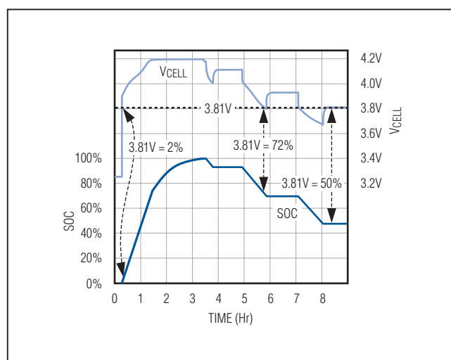
Figure 3. Instantaneous Voltage Does Not Translate Directly to SOC
