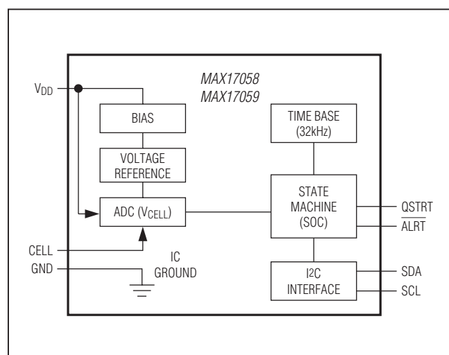
Figure 2. Block Diagram
