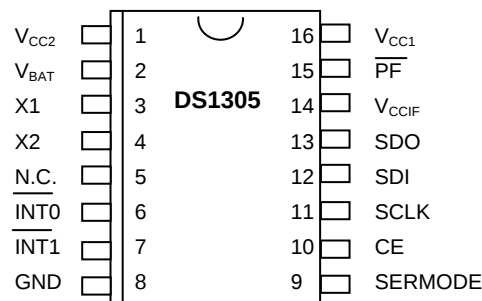
DIP (300 mils)
