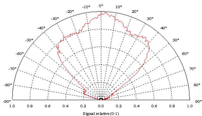
RADIATION PATTERN
