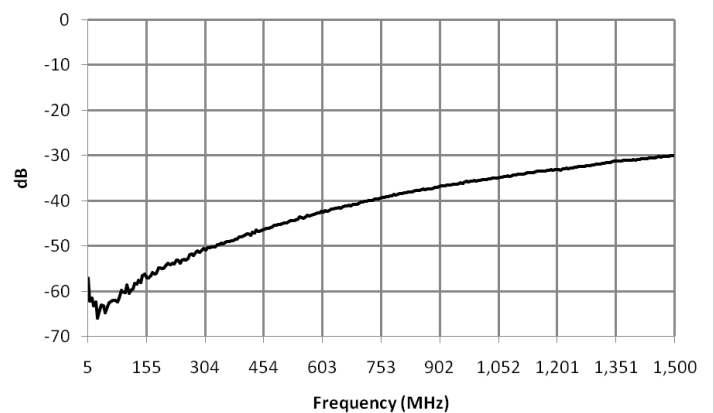
Isolation (Pin6-3)
