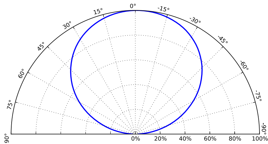
Figure 7. Typical polar radiation pattern for L1MX-xxxxxxxxxx0 at test current, T_j=85^{\circ}\text{C} .
