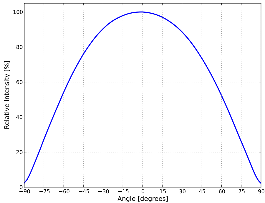
Figure 6. Typical radiation pattern for L1MX-xxxxxxxxxx0 at test current, T_j=85^{\circ}\text{C} .
