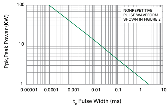
Figure 3. Surge Derating Curve
