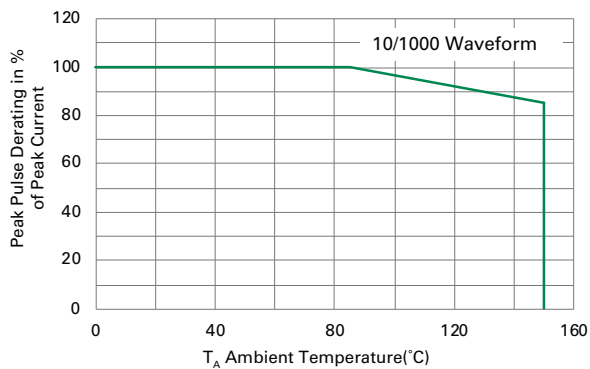
Figure 3. Surge Derating Curve
