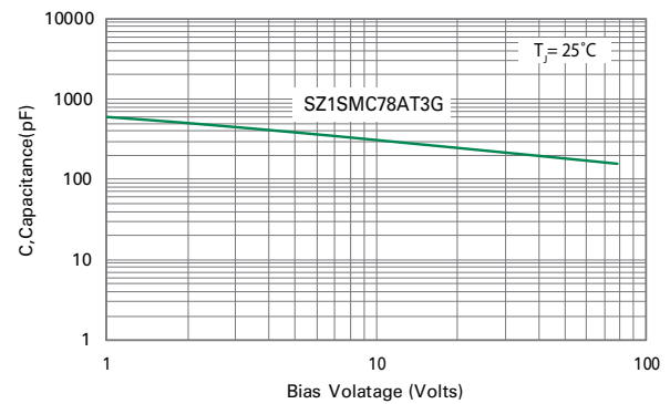
Figure 4. Typical Junction Capacitance vs. Bias Voltage
