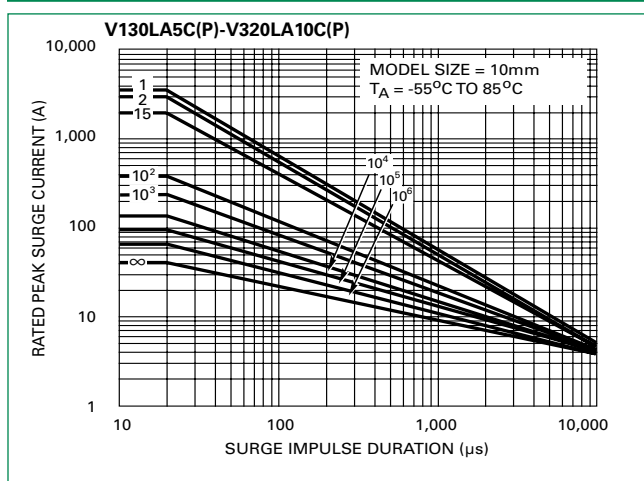
Figure 4. Repetitive Surge Capability for 10mm Parts
