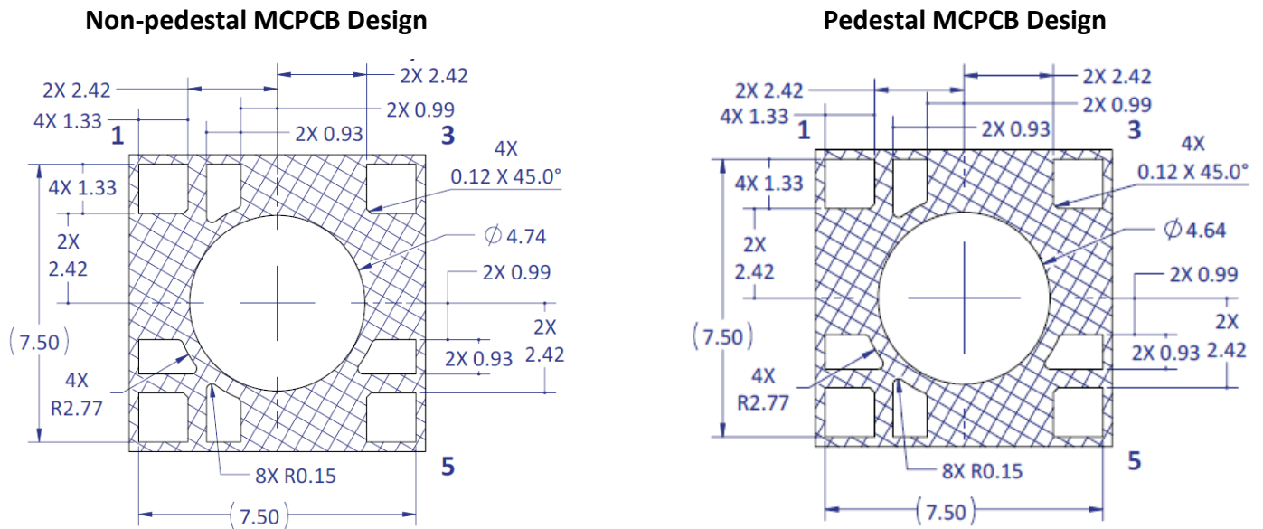
Figure 2c: Recommended 8mil stencil apertures layout for anode, cathode, and thermal pad for non-pedestal and pedestal design
