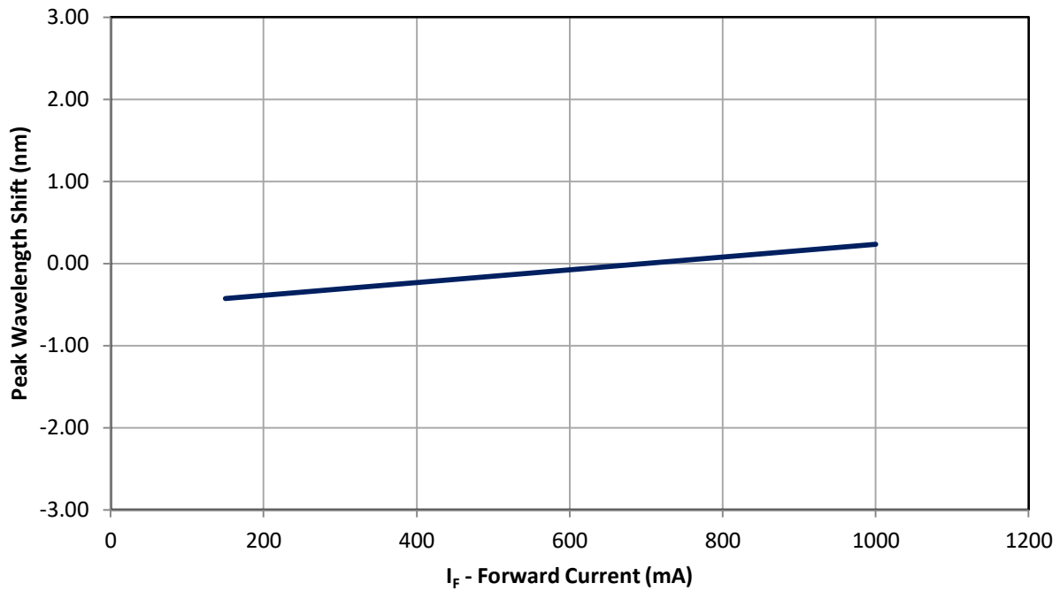
Figure 9: Typical peak wavelength shift vs. forward current @ T_c = 25^\circ\text{C}
