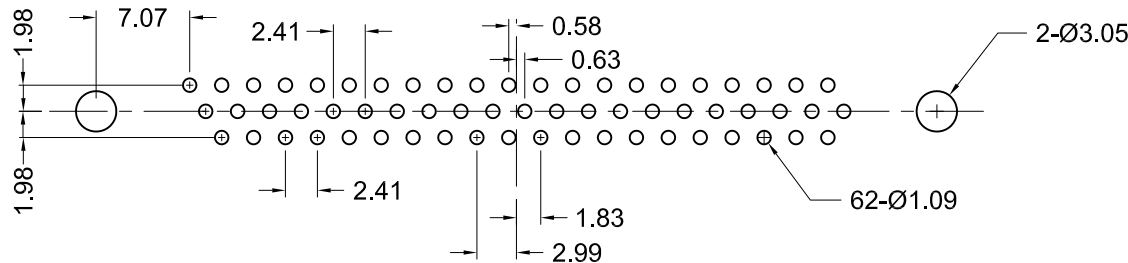
Recommended PCB Layout (Top View)
