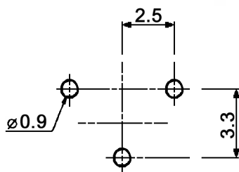
HOLE LAYOUT TOP VIEW \pm 0.05
