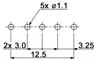
HOLE LAYOUT TOP VIEW
