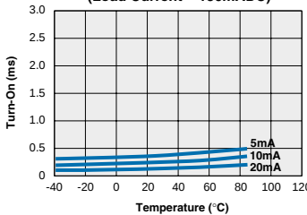
TS190 Typical Turn-On vs. Temperature (Load Current = 150mADC)
