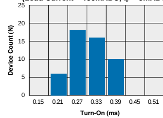
TS190 Typical Turn-On Time (N=50 Ambient Temperature = 25°C) (Load Current = 150mADC; I_F = 5\text{mADC} )
