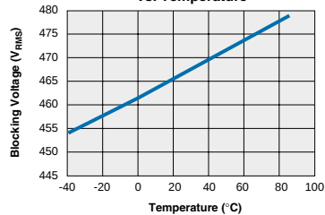
TS190 Typical Blocking Voltage vs. Temperature
