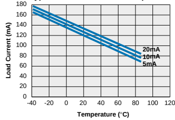
TS120 Typical Load Current vs. Temperature
