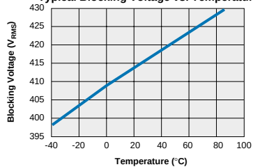
TS120 Typical Blocking Voltage vs. Temperature
