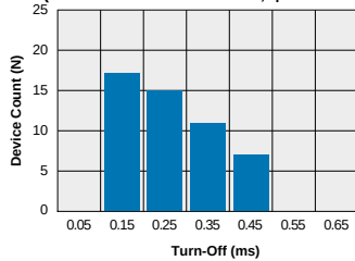
TS120 Typical Turn-Off Time (N=50 Ambient Temperature = 25°C) (Load Current = 120mA; I_F = 5\text{mA} )
