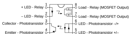
TS117/TS117L Pinout
