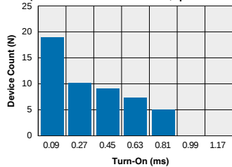
IBB110P Typical Turn-On Time (N=50 Ambient Temperature = 25°C) (Load Current = 100mADC; I_F = 5\text{mADC} )
