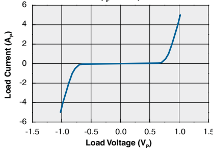
Typical Load Voltage vs. Load Current ( I_F = 5\text{mA} )
