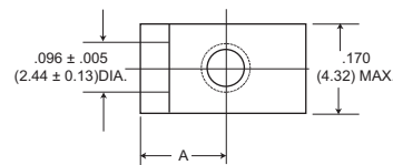
90° Angle Mounting Bracket
