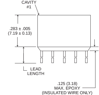
Plug
