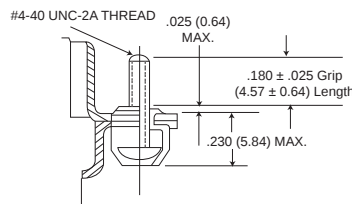
Low Profile (F173) Jackcrew (factory installed)
