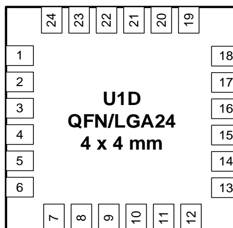
Figure 1D: U1D (QFN/LGA24_4x4 mm)
