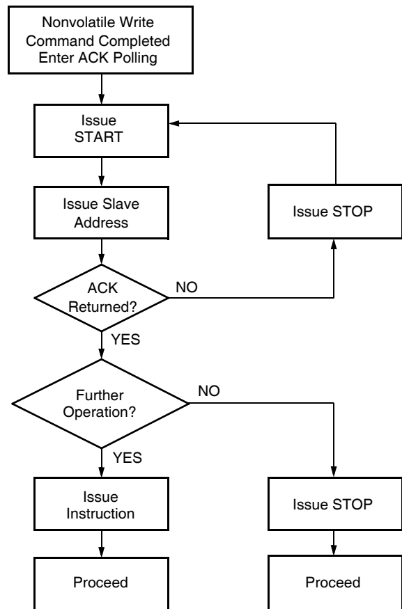
Flow 1. ACK Polling Sequence
