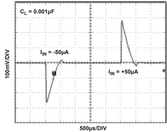
FIGURE 24. 50μA LOAD TRANSIENT RESPONSE
