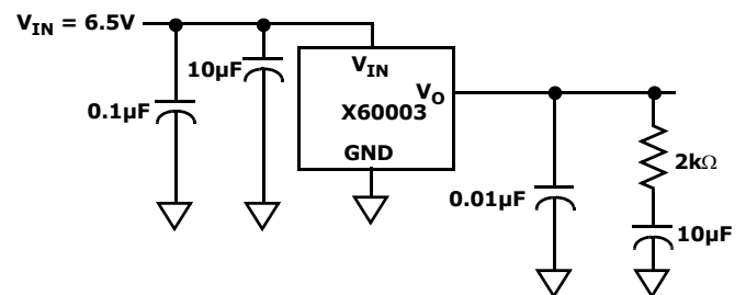
FIGURE 35. NOISE REDUCTION NETWORK
