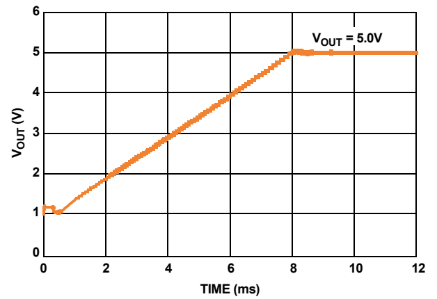
FIGURE 31. TURN-ON TIME
