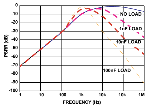
FIGURE 22. PSRR vs CAP LOAD
