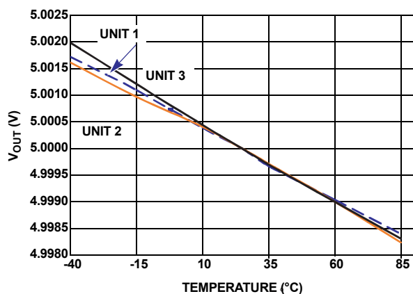
FIGURE 21. V_{OUT} vs TEMPERATURE (3 UNITS)
