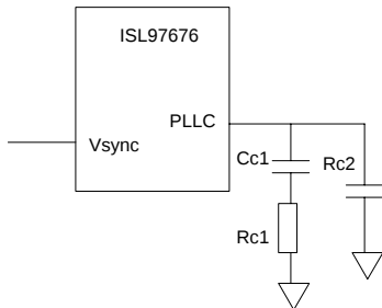
FIGURE 24. PLL CONFIGURATION
