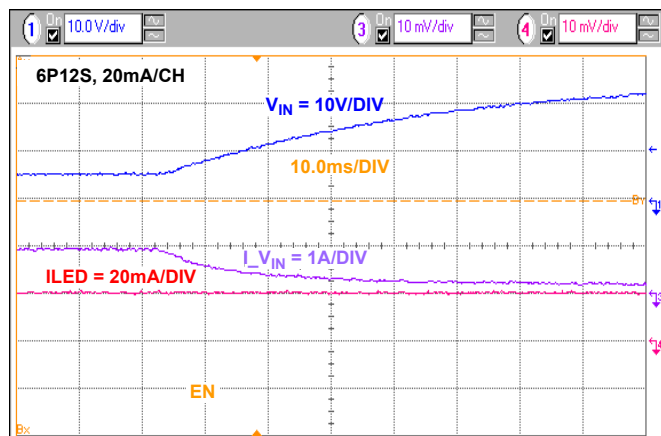
FIGURE 14. LINE REGULATION WITH V_{IN} CHANGE FROM 6V TO 26V, V_{IN} = 12V , 6P12S AT 20mA/CHANNEL
