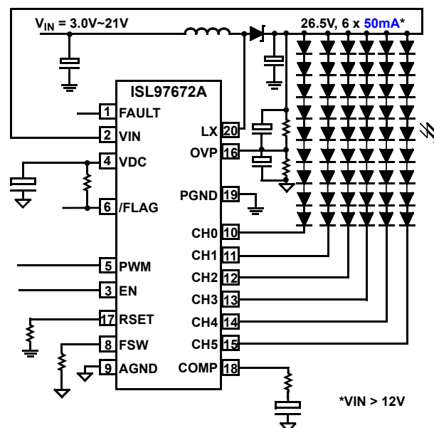
FIGURE 24. SINGLE SUPPLY 3.0V OPERATION
