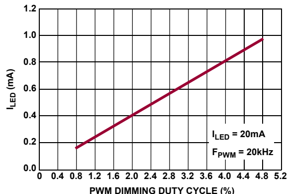
FIGURE 20. MINIMUM DIMMING LINEARITY AT 20kHz
