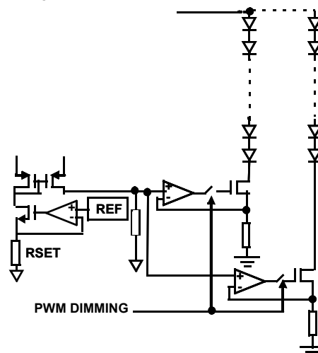
FIGURE 21. SIMPLIFIED CURRENT SOURCE CIRCUIT
