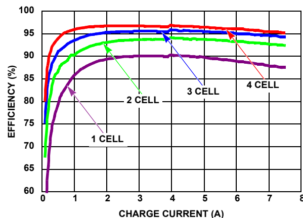
FIGURE 8. EFFICIENCY vs CHARGE CURRENT AND BATTERY VOLTAGE (EFFICIENCY \text{DCIN} = 20\text{V} )
