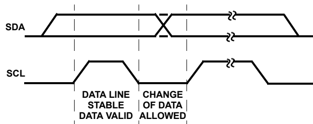
FIGURE 22. DATA VALIDITY
