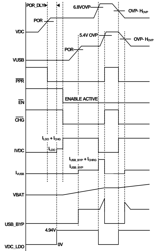
FIGURE 2. CHARGING PROFILE
