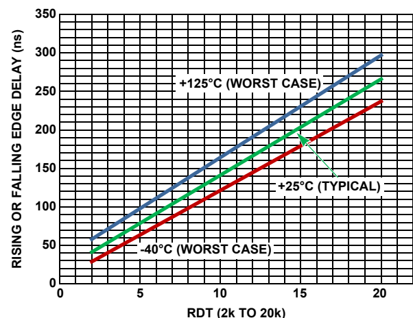
FIGURE 2. PROGRAMMABLE TIME DELAYS
