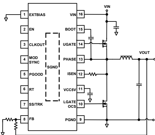
FIGURE 1. TYPICAL APPLICATION
